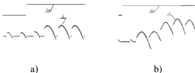
Fig. 1. The reaction of the current circuit to the jump of the task: a) from one value of the intermittent mode to another; b) from intermittent to continuous current mode.
