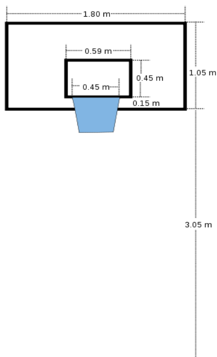
Physical dimensions of the basketball backboard Marking and baskets on it
