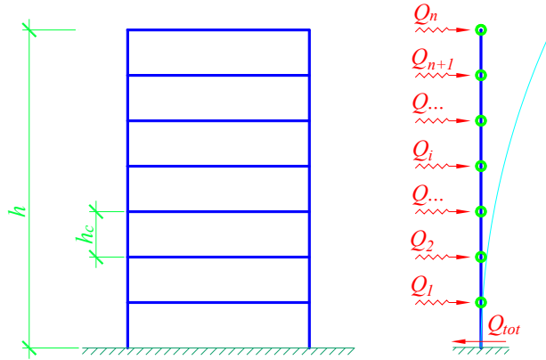
Fig. 1. The scheme of the cantilever five-storey building: a) geometric scheme, b) dynamic calculation scheme
