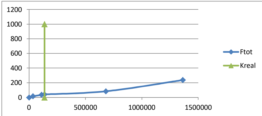
Fig. 4. Graph of the dependence F_{tot}(k) in the range of real stiffness, for which the system of equations (3) has been solved
