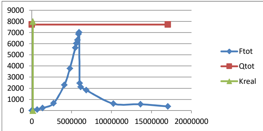
Fig.3. Graph of the dependence F_{tot}(k) in the whole range of stiffness, for which the system of equations (3) has been solved
