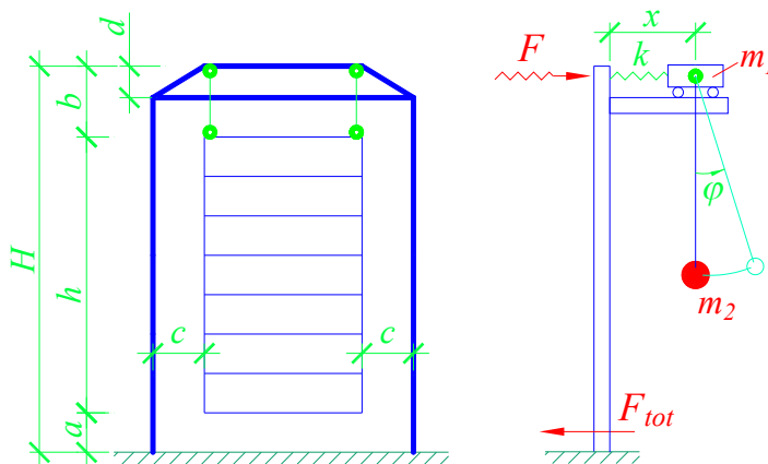
Fig.2. Scheme of the suspended fifteen-story building: a) geometric scheme; b) dynamic calculation scheme
